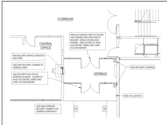
Proposed Floor Plan
