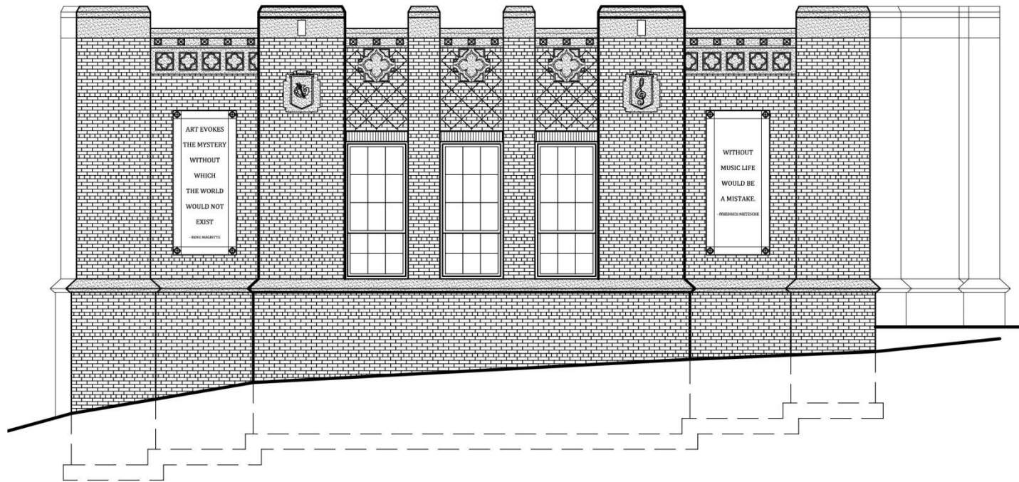
OYSTER BAY HIGH SCHOOL NORTH ELEVATION (LAWN at 3D ART ROOM)
