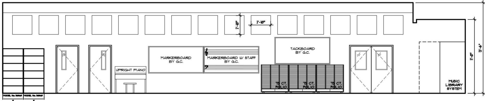
BAND ROOM FRONT ELEVATION
